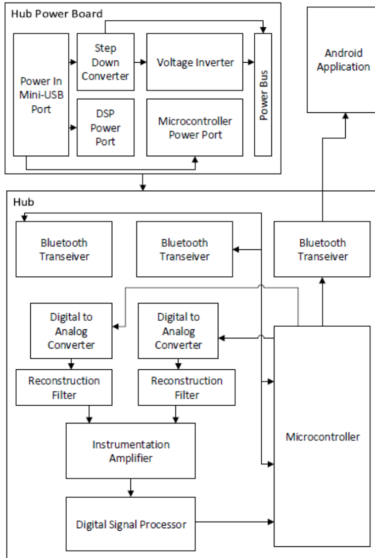
Figure 5.2- External processing and charging hub
