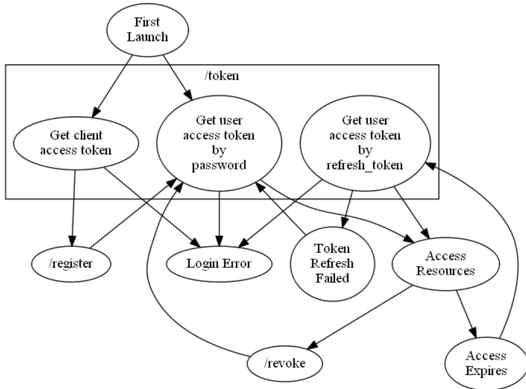
Figure 7.1.2 - Authentication Flow
