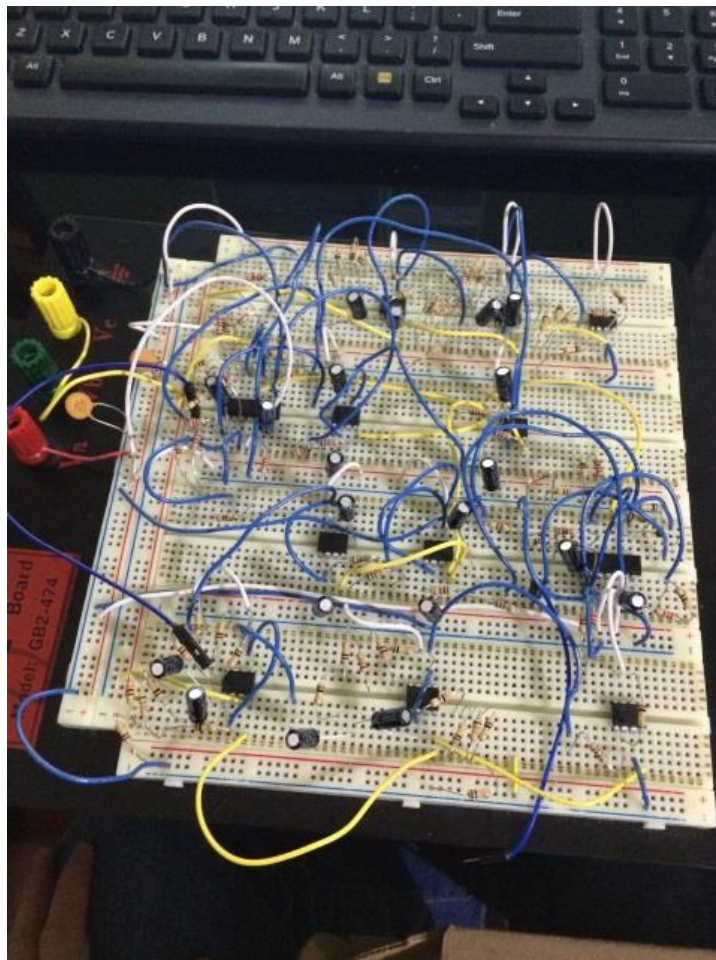
Figure 9.6.1 – Breadboard Sensors
