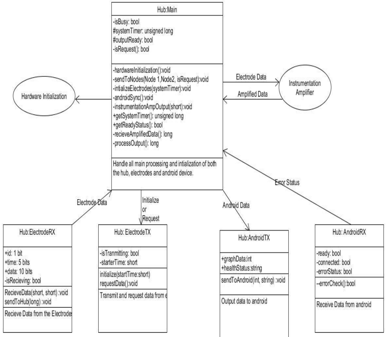
Figure 5.3.2.2-Hub UML diagram
